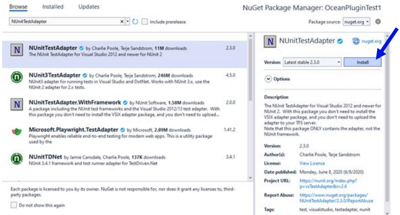
Figure 2: Install NUnitTestAdapter package
